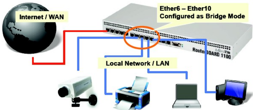
Gambar 7.1 System bridge
