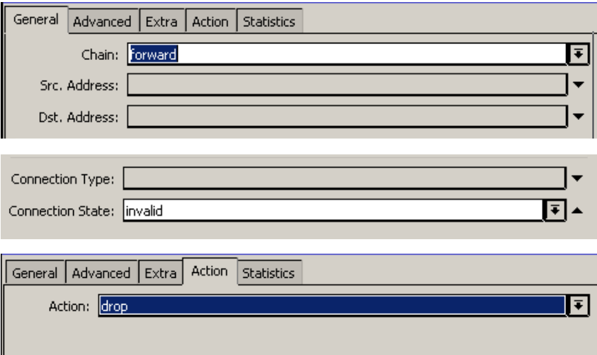
Gambar 3.19 Connection state rule
