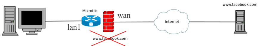
Gambar 3.10 Diagram firewall block host
