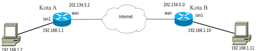
Gambar 8.1 EoIP tunnel
