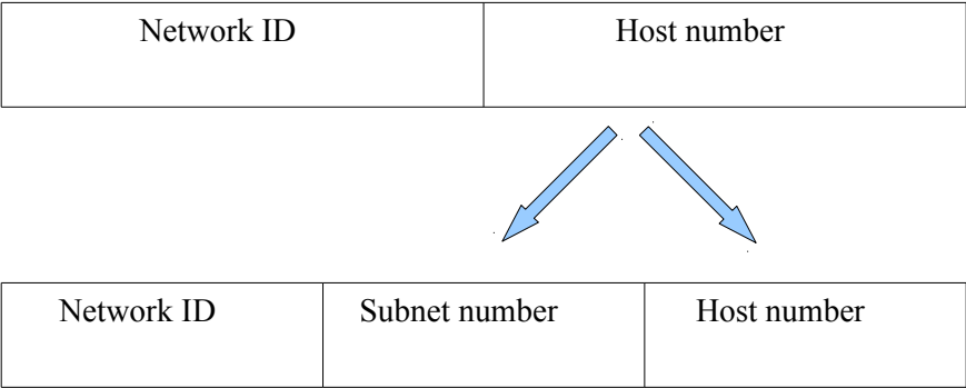
Gambar 1.4 Hirarki Subnet Address
