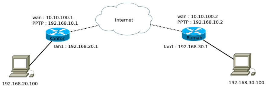
Gambar 8.10 PPTP Tunnel
