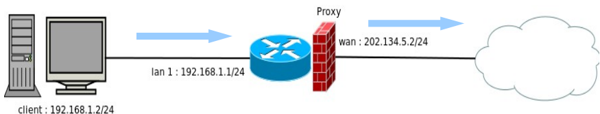
Gambar 3.1 Diagram blok proxy
