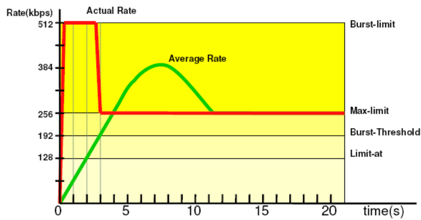
Gambar 5.15 Diagram burst
