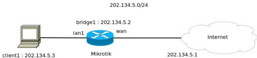
Gambar 7.3 Lab bridge
