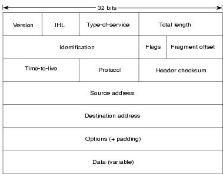
Gambar 1.3 Paket IP
